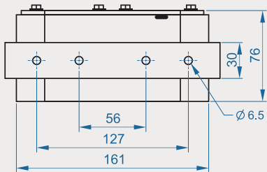
MOUNTING HOLES
